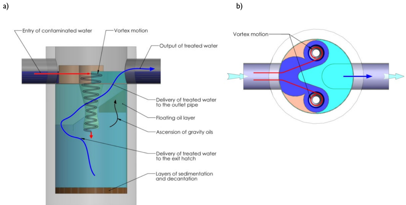
Figure 1. a) Cross sectional and b) Top view flow diagrams of NEXT Stormwater Solutions' SDD3 oil-grit separator technology.
